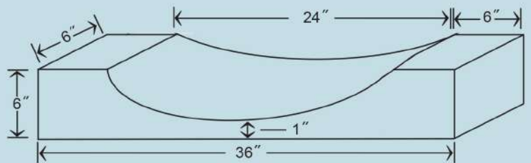
Drawing not to exact scale
